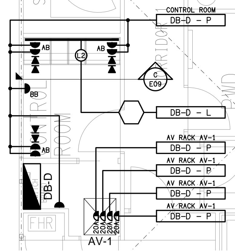
DETAIL A ELECTRICAL CONTROL ROOM SCALE 1:50
